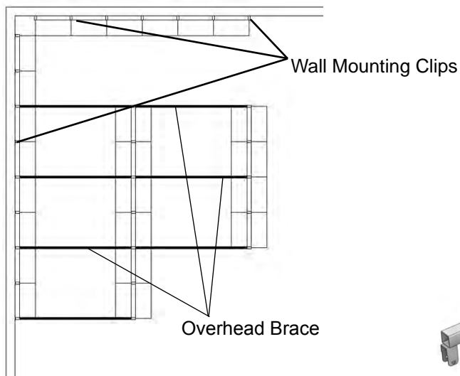
Recommended locations for Overhead Braces/Wall Mount Clips.
